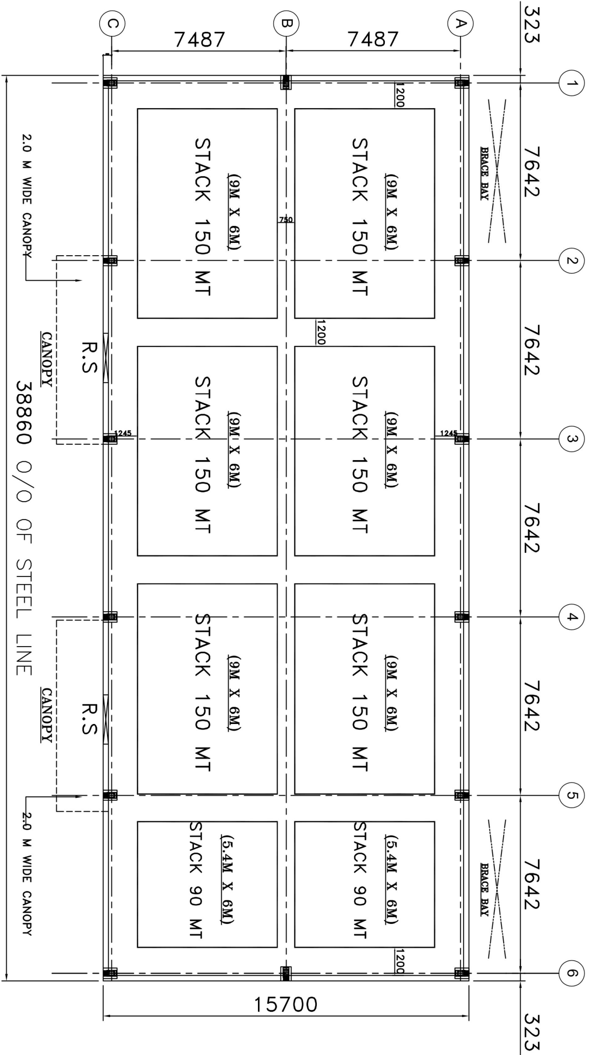
LAYOUT PLAN
