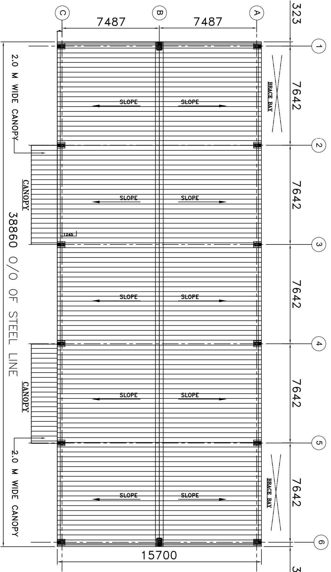
ROOF LAYOUT PLAN
